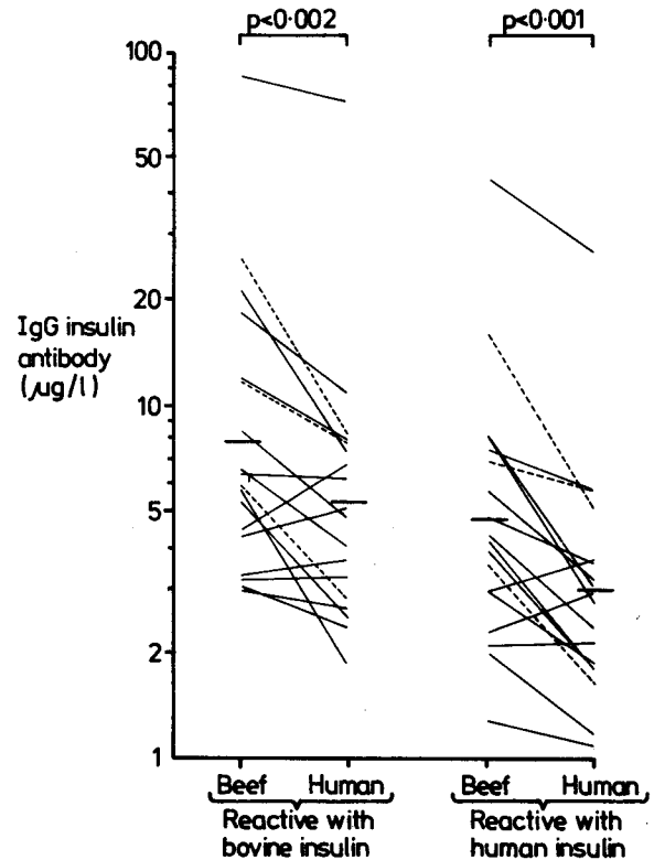
FIG 4—Bovine and human insulin antibody binding concentrations after six weeks' treatment with beef and human ultralente insulin in random order. Horizontal bars denote geometric mean values. Dotted lines indicate the three patients in whom the dose of human ultralente insulin was reduced because of hypoglycaemia.
